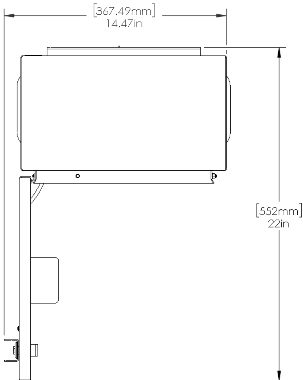
Figure F – Cabinet Footprint
