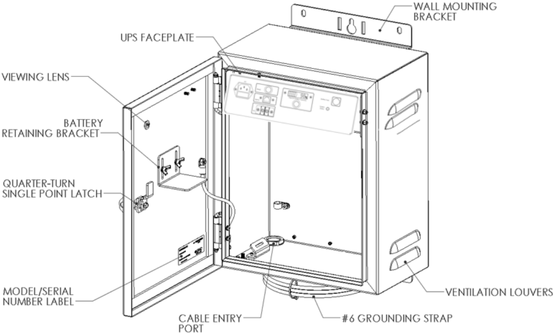
Figure B – Front View of Cabinet w/ Door Open
