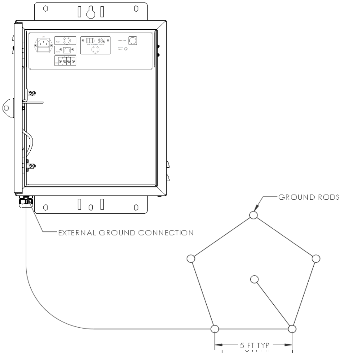
Figure G – Grounding Diagram
