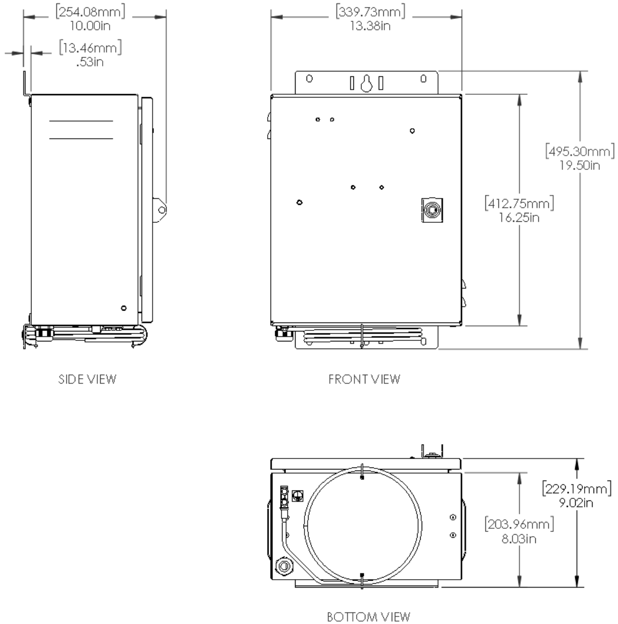
Figure D – Cabinet Overall Dimensions
