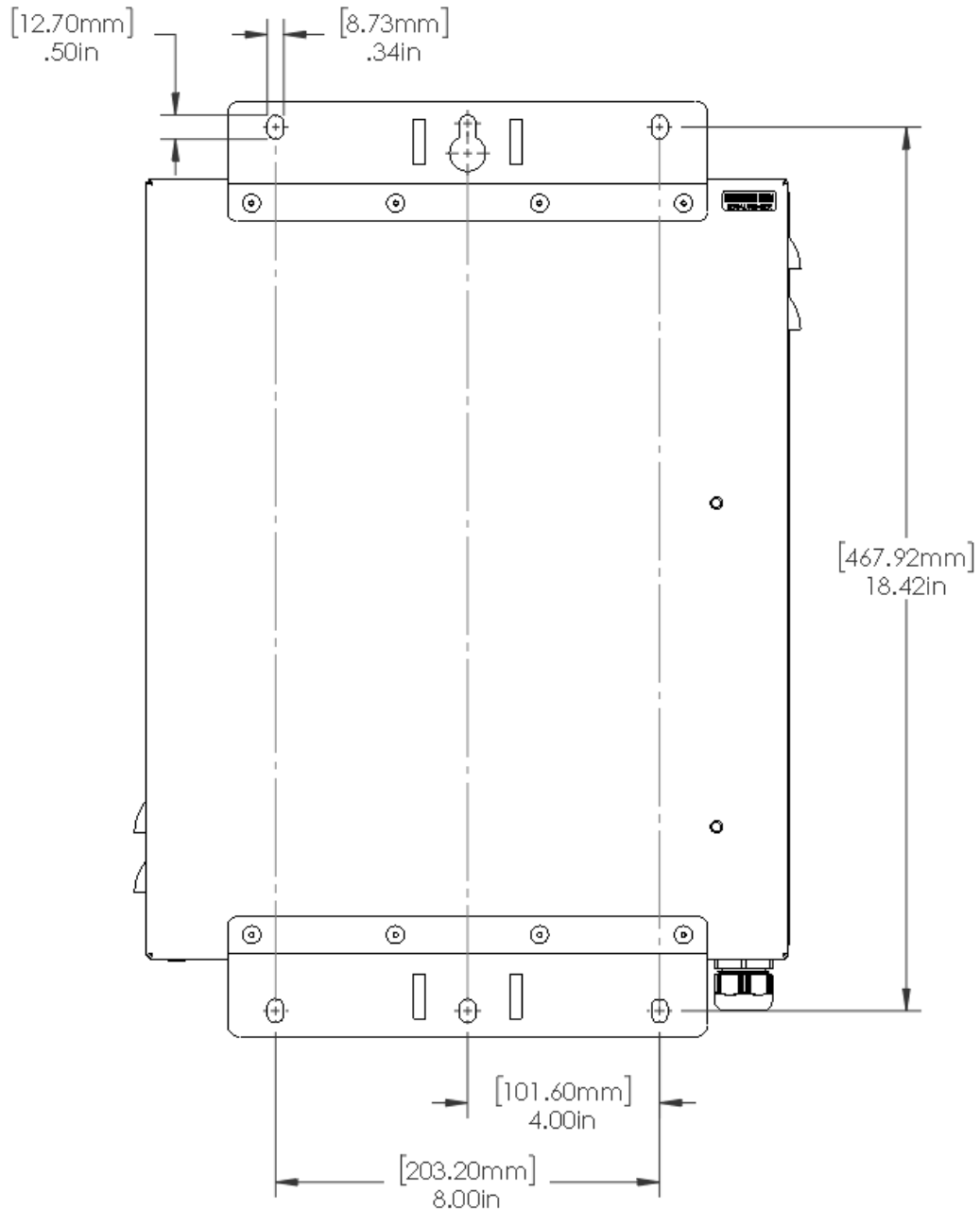
Figure E – Cabinet Mounting
